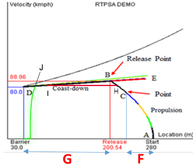
FIGURE 18: Uniform motion in original RTPSA, schematic diagram.
