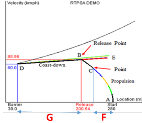
FIGURE 7: Coast-down module, from B to D[18].
